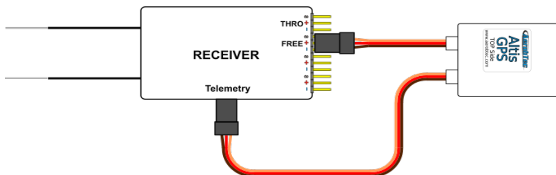
Fig 4: Telemetry connection
