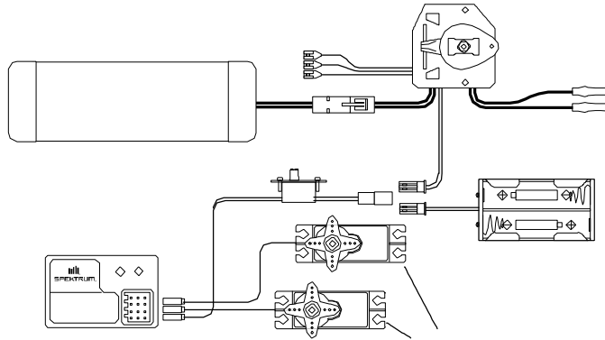
Figure A – Connections to B.E.C. and receiver with mechanical speed controller. Ni-Cd battery and speed controller are not included in the radio set.
